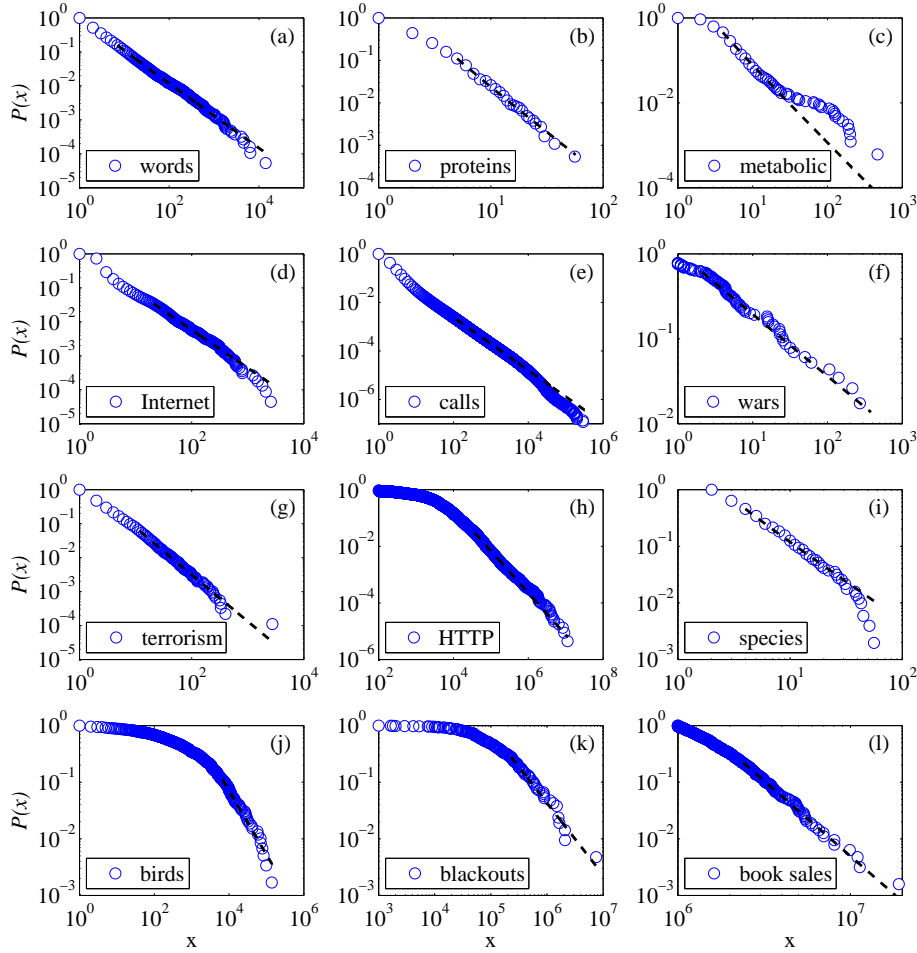
FIG. 6.1. The cumulative distribution functions P(x) and their maximum likelihood power-law fits for the first twelve of our twenty-four empirical data sets. (a) The frequency of occurrence of unique words in the novel Moby Dick by Herman Melville. (b) The degree distribution of proteins in the protein interaction network of the yeast S. cerevisiae . (c) The degree distribution of metabolites in the metabolic network of the bacterium E. coli . (d) The degree distribution of autonomous systems (groups of computers under single administrative control) on the Internet. (e) The number of calls received by US customers of the long-distance telephone carrier AT&T. (f) The intensity of wars from 1816–1980 measured as the number of battle deaths per 10 000 of the combined populations of the warring nations. (g) The severity of terrorist attacks worldwide from February 1968 to June 2006, measured by number of deaths. (h) The number of bytes of data received in response to HTTP (web) requests from computers at a large research laboratory. (i) The number of species per genus of mammals during the late Quaternary period. (j) The frequency of sightings of bird species in the United States. (k) The number of customers affected by electrical blackouts in the United States. (l) The sales volume of bestselling books in the United States.
