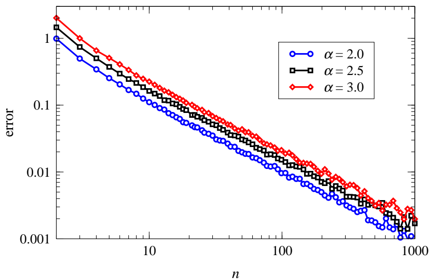
FIG. B.2. The error on the estimated scaling parameter \hat{\alpha} from sample size effects for continuous data (similar results hold for the discrete case), for \alpha = 2, 2.5, and 3 (for 100 repetitions), as a function of sample size. The average error decays as O(n^{-1}) and becomes smaller than 1% of the value of \alpha when n \gtrsim 50 .
